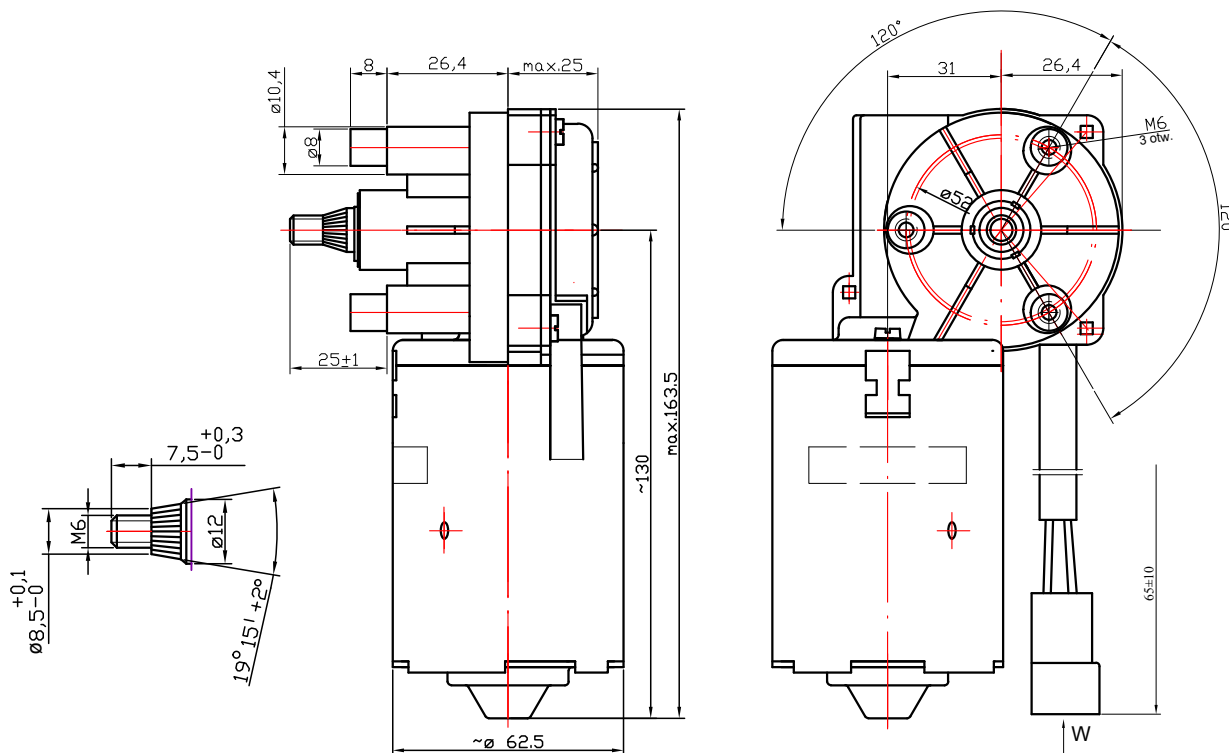
Widok "W"
